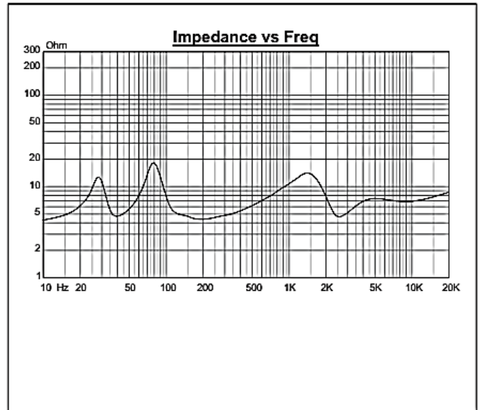
Impedance and Phase Curves
