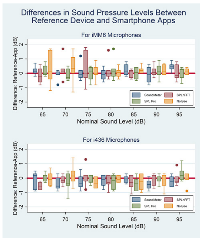
Fig. 2. (Color online) (a) Box plots of differences [difference (SPL) = reference output – app output] between measurements by the reference system and by smartphone apps by nominal sound levels for iMM-6 microphones (top), and (b) box plots of differences for i436 microphones (bottom).
